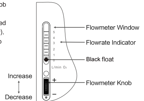
Figure 7: Setting Flowrate
